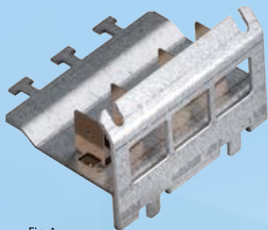
Fig. 1 VarioLine® UF AP3-MC45E adapter plate for max. 3 MC45 modules (in ELine format)
